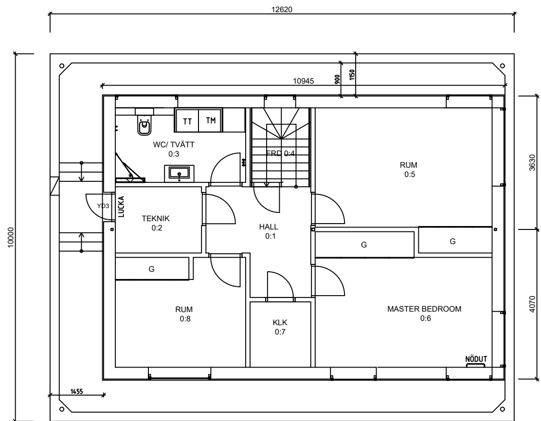
PLAN 0 KASSUNPLAN, ca 72 kvm SKALA 1:100
